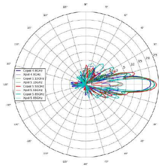
Elevation Vertical
