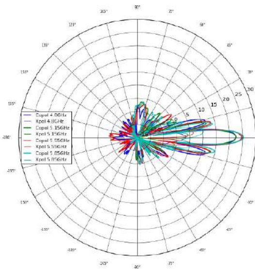
Elevation Horizontal
